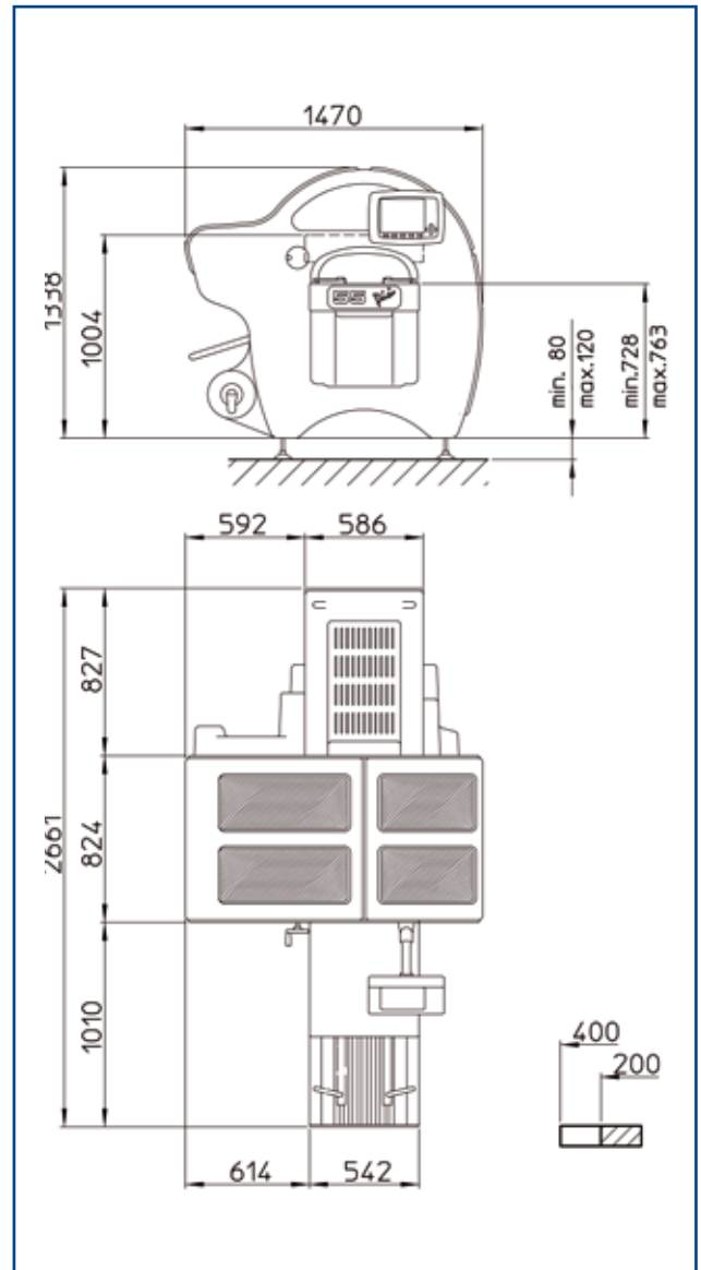
Technical drawing
